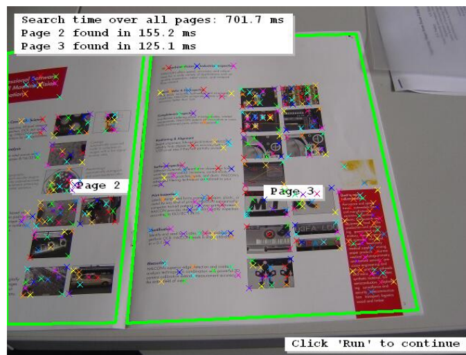
Figure 10.8: Different pages of a HALCON brochure are located via descriptor-based matching.
