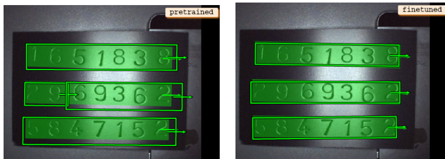
Figure 19.6: The retrained model improved the localization of numbers (right) compared to the pretrained model (left).
