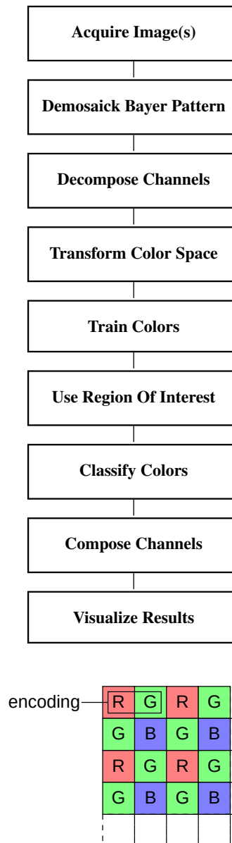
Figure 14.3: Sample Bayer pattern and corresponding encoding.
