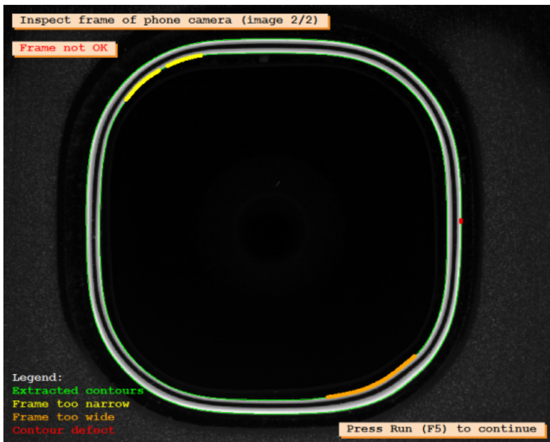
Figure 9.6: Image of the camera frame of a phone together with the extracted and classified edges.
