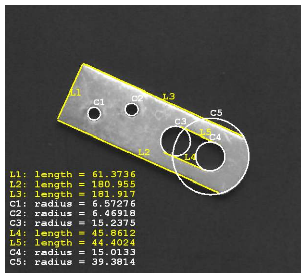
Figure 9.4: Fitted lines and circles.
