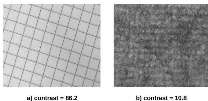
Figure 15.20: Contrast values of a) grid and b) dust filter.
