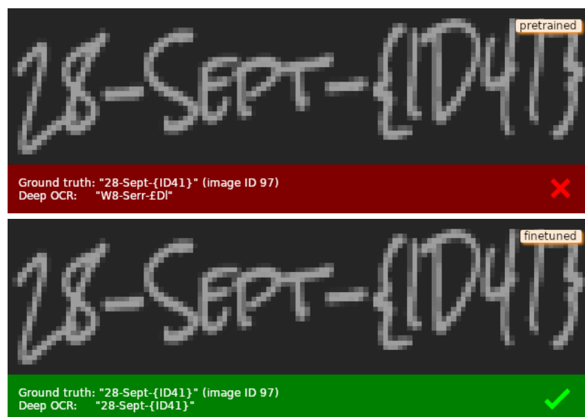
Figure 19.5: The retrained model learned to identify the font and characters (bottom) it could not handle correctly before (top).
