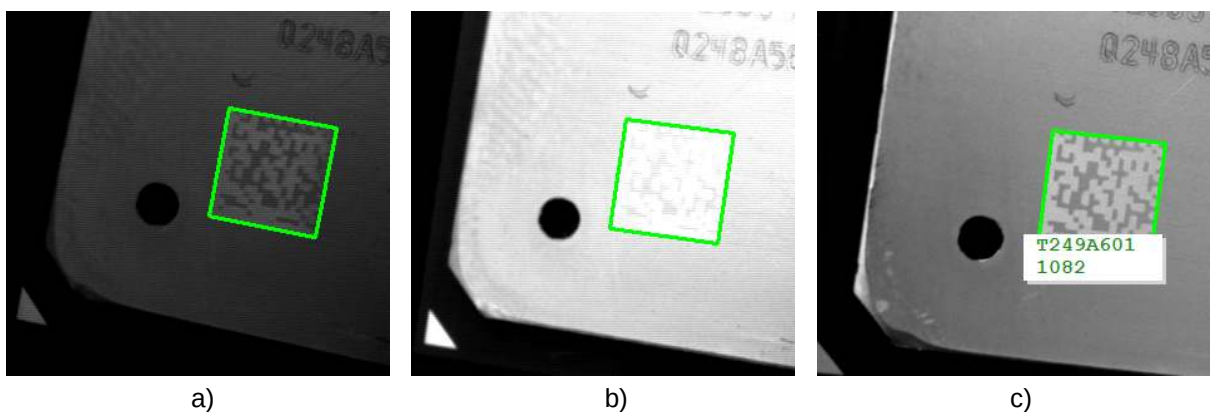
Figure 17.2: (a) Dark training image; (b) bright training image; (c) read code.
